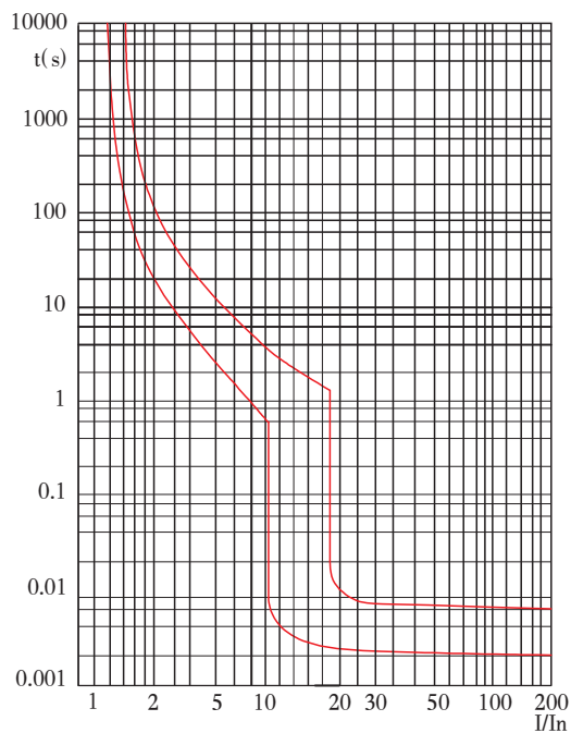
D型 type CH3N-63, CH3H-63, CH3LN-40, CH3LN-63, CH3LH-63
