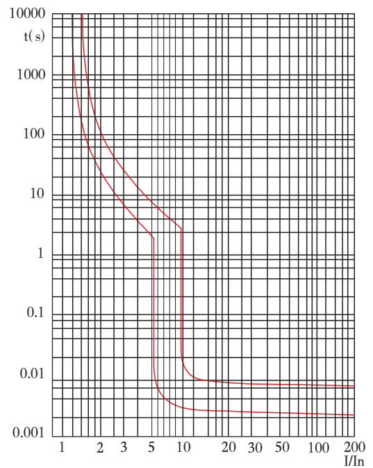
C型 type CH3N-40, CH3N-63, CH3H-63, CH3LNN-32, CH3LN-40, CH3LN-63, CH3LH-63
