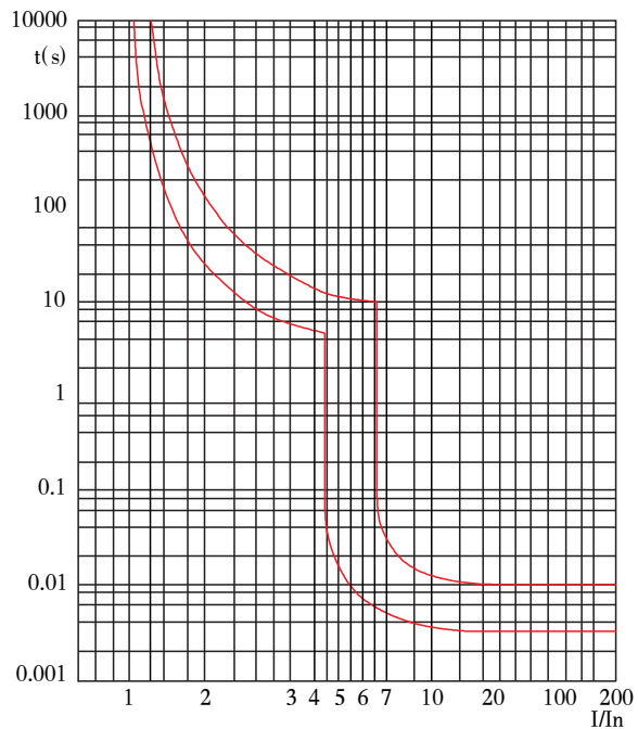
B型 type CH3Z-63
